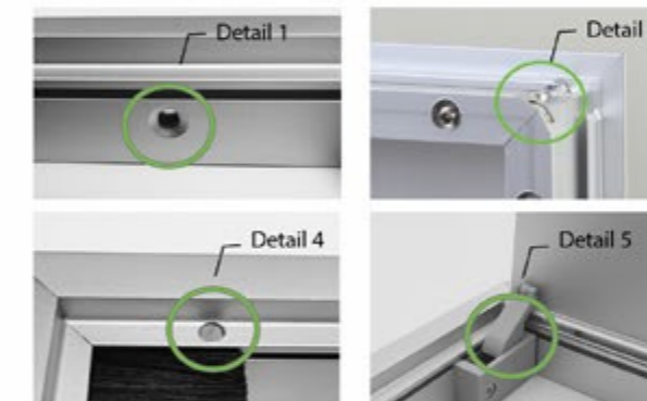
Detail 2: Brush to hide cables Detail 3: Radius 8 for easy cut out Detail 5: Spring mechanism (for width 100 mm upwards on demand)
