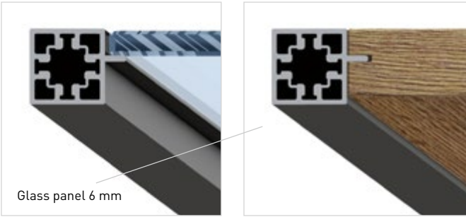
Profile for glass panels 6 mm 82794.*** Can also be used for the assembly of wooden panels with peripheral groove. (See also page 12)
