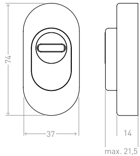
Design escutcheon made of stainless steel with pull protection, anti-drilling protection and height adjustment
